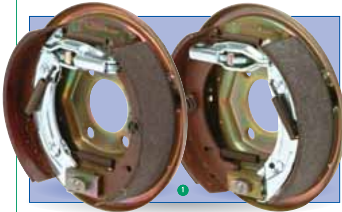
1 P000140 Brake assembly, 200 x 50 RH & LH - Bolt on type backplates pre-assembled with shoes, springs etc (From Jan 1996). £73.95
