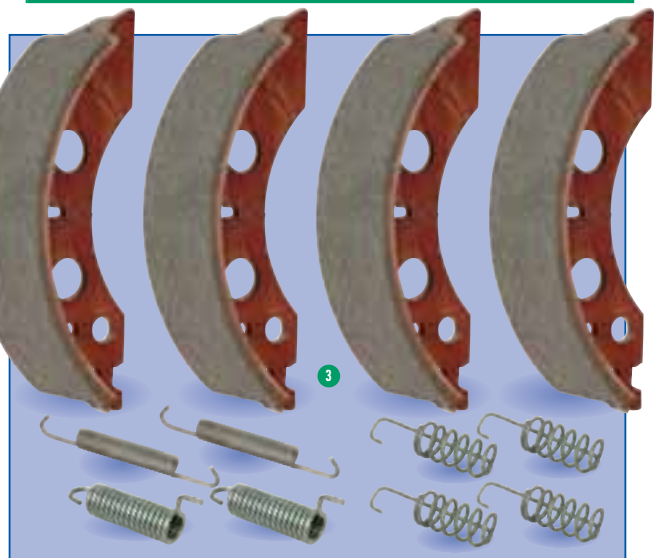
3 P00860 Brake shoe set. 2051 brake (will also fit 2050 brake). £49.50 A full set comprising of four brake shoes and all springs required to complete the installation. This kit services one axle, for continued safety, brakes should always be changed as complete axle sets.
