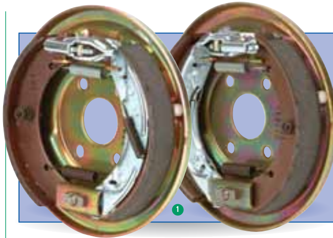
1 P000160 Brake assembly. 250 x 40 RH & LH - Bolt on type backplates pre-assembled with shoes, springs etc (From Jan 1996). £111.95
