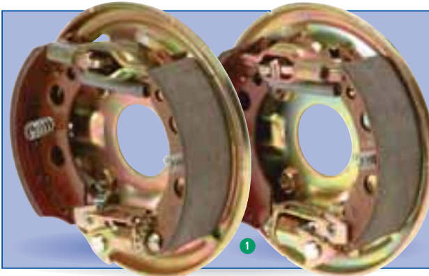
1 P00060 Complete 2050 brake assembly (Axle Set). Pre-fitted to backplate and complete with all springs, adjusters etc... £109.95
